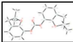
Fig. 1. Perspective view of one the the three molecules of the title compound showing 30% probability displacement ellipsoids.
